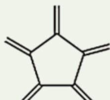
[5]轴烯 (c)
