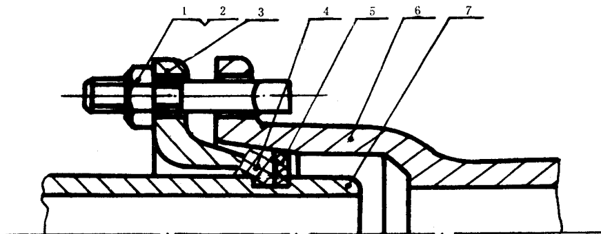
(a) N型接口简图
